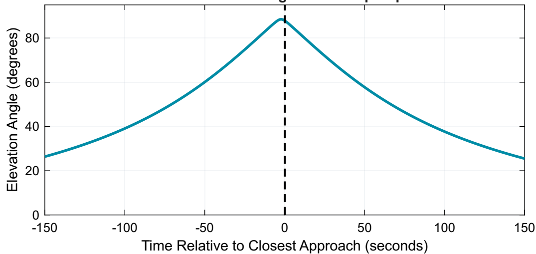
Satellite Elevation Angle from UE perspective
