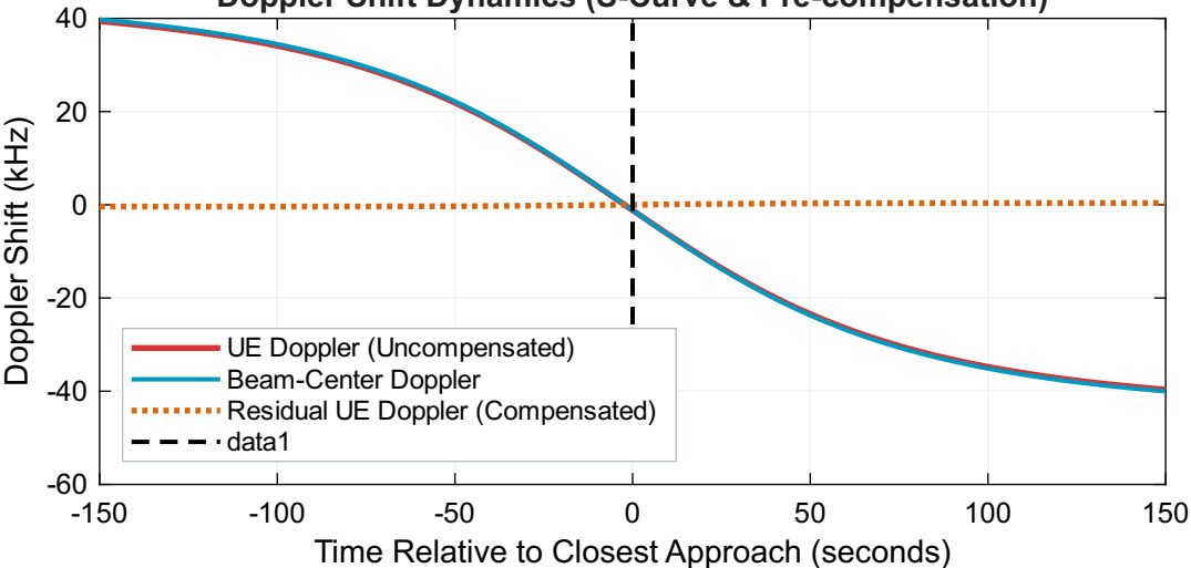
Doppler Shift Dynamics (S-Curve & Pre-compensation)
